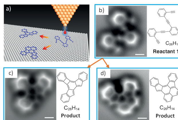
Figure 1. a) The tip apex was functionalized with a CO molecule for imaging of the reactant and the final products on the metal surface. b) AFM image of the reactant 1,2-bis[(2-ethynylphenyl)ethynyl]benzene. c, d) Two representative products that were observed after the sample had been heated to 90 °C. [1d] Scale bars: 0.3 nm.
